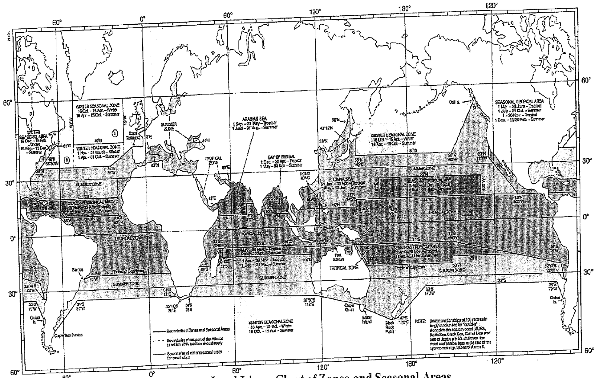
Load Line - Chart of Zones and Seasonal Areas
